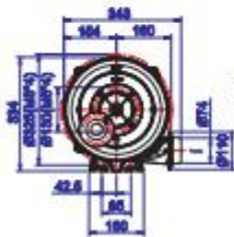
HTB75-105 5-stage
