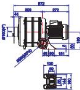
HTB75-104 4-stage
