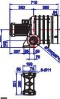
HTB100-505 5-stage
